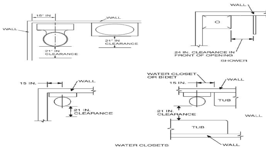
FIGURE R307.1 MINIMUM FIXTURE CLEARANCES
